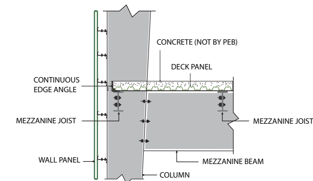
Mezzanine Beam Connection to Main Frame Column
