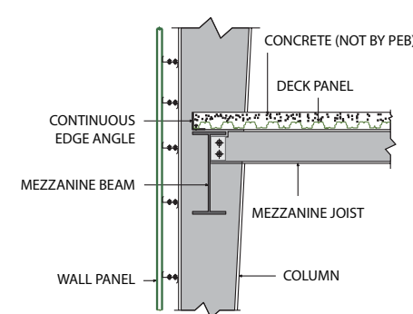
Mezzanine Joist Connection to Mezzanine Beam
