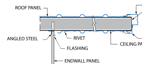
Endwall Roof Extension With Soffit
